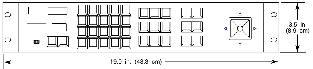
V1300X-RVC Rack-Mounted Keypad
