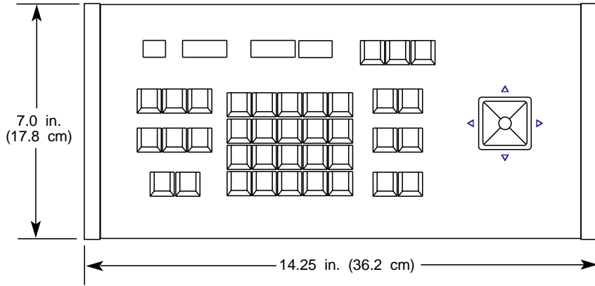
V1300X-DVC Desk-Top Keypad
