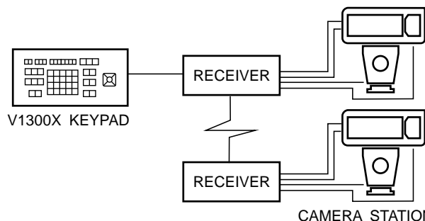
Figure 3-a V1300X Keypad Used as Diagnostic Device for Matrix 44 Switcher
