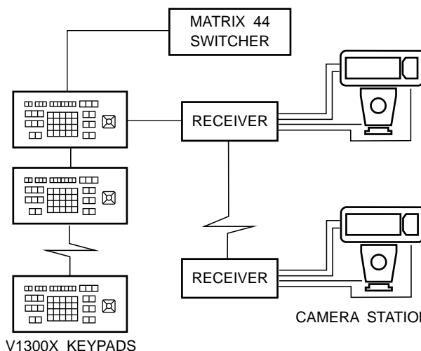
Figure 3-c Multiple V1300X Keypads Used in Standalone Mode
