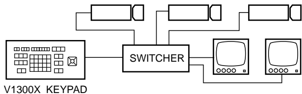
Figure 3-a V1300X Keypad Used as Diagnostic Device for Matrix 44 Switcher
