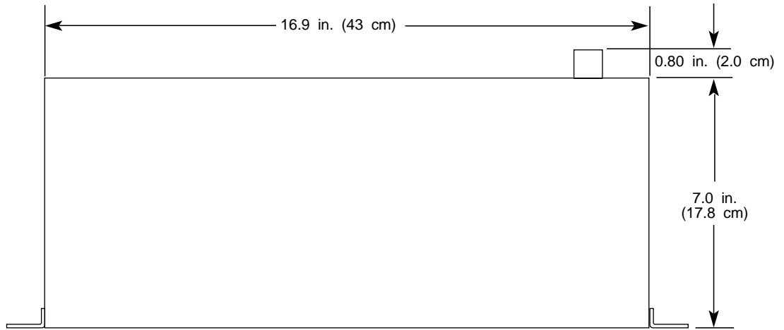
V1300X-DVC Desk-Top Keypad
